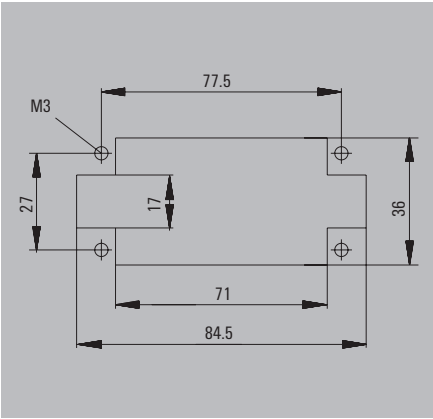
Installation cut-out
