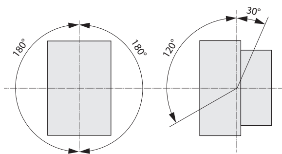
Figure 74 - 100-E116K..., 100-E146K... Contactors
