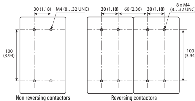
Figure 77 - Drilling Template for 116...146 A 3-Pole Contactors
