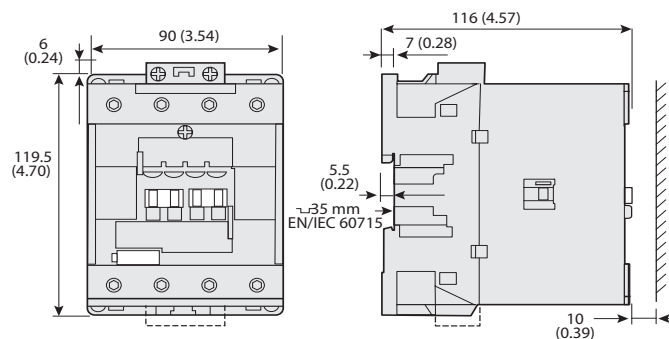
Figure 71 - 100-E80 4-Pole Contactors
