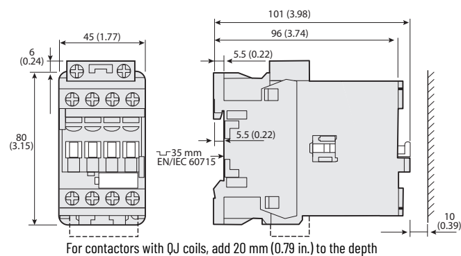
Figure 44 - 100-E26...100-E38 4-Pole Contactors with Standard Coils
