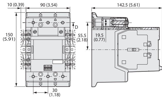
Figure 78 - 104-E116E..., 104-E146E... Reversing Contactors with Cat. No. 100-EM... Mechanical Interlock
