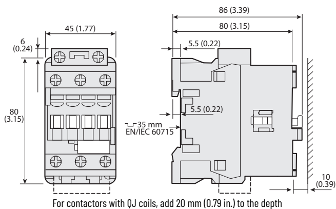
Figure 43 - 100-E26...100-E38 3-Pole Contactors with Standard Coils
