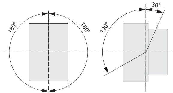
Figure 76 - 100-E116K..., 100-E146K... Contactors
