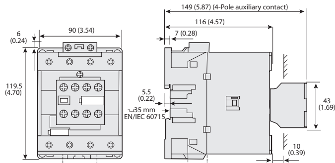
Figure 72 - 100-E80 4-Pole Contactors with Front-mounted Auxiliary Contact
