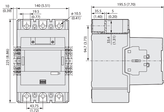
Figure 85 - 100-E265E...100-E370E Contactors with PLC Input
