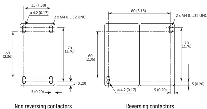
Figure 56 - Drilling Template for 26...38 A Contactors
