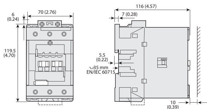
Figure 67 - 100-E80...100-E96 3-Pole Contactors with Front-mounted Auxiliary Contact
