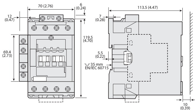
Figure 64 - 100-E40...100-E52 4-Pole Contactors with Side-mounted Auxiliary Contact
