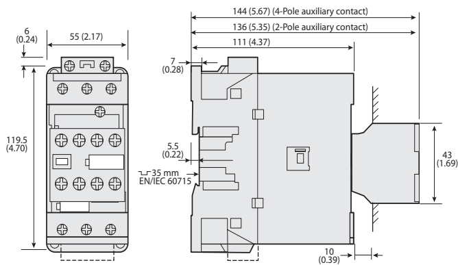
Figure 59 - 100-E40...100-E65 3-Pole Contactors with Side-mounted Auxiliary Contact
