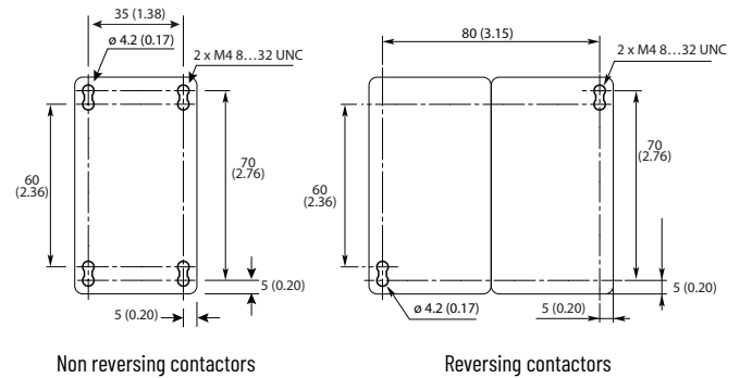
Figure 62 - 100-E40...100-E52 4-Pole Contactors
