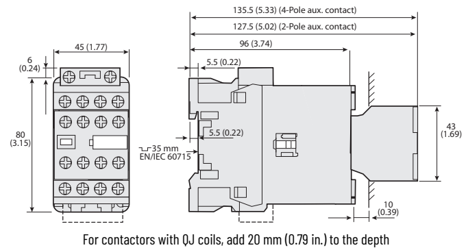
Figure 49 - 100-E26...100-E38 3-Pole Contactors with Standard Coils and Side-mounted Auxiliary Contact
