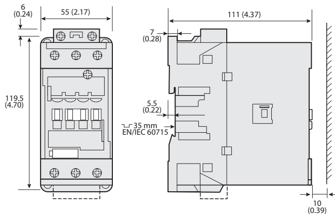
Figure 57 - 100-E40...100-E65 3-Pole Contactors
