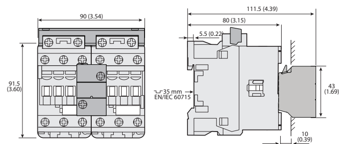
Figure 55 - 104-E26...104-E38 Reversing Contactors with Cat. No. 100-EMCA02 Mechanical and Electrical Interlock
