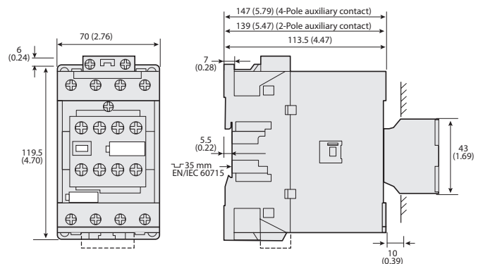
Figure 63 - 100-E40...100-E52 4-Pole Contactors with Front-mounted Auxiliary Contact
