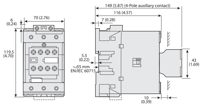
Figure 68 - 100-E80...100-E96 3-Pole Contactors with Side-mounted Auxiliary Contact
