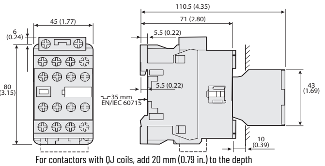
Figure 38 - 100-E09...100-E16 Contactors with Standard Coils and Side-mounted Auxiliary Contact
