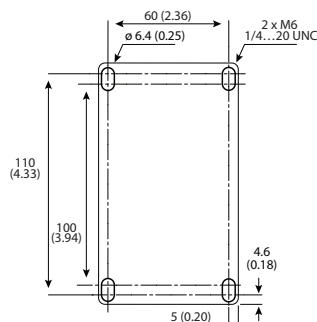
Figure 65 - Drilling Template for 40...52 A 4-Pole Contactors
