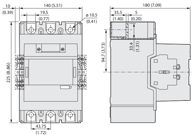
Figure 84 - 100-E265...100-E370 Contactors
