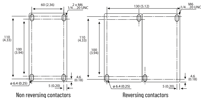
Figure 71 - 100-E80 4-Pole Contactors
