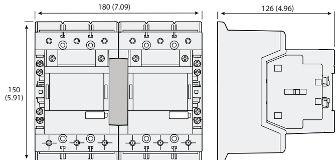
Figure 78 - 104-E116E..., 104-E146E... Reversing Contactors with Cat. No. 100-EM... Mechanical Interlock
