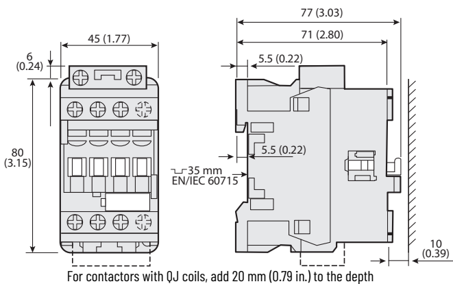
Figure 36 - 100-E09...100-E16 Contactors with Low-consumption Coils
