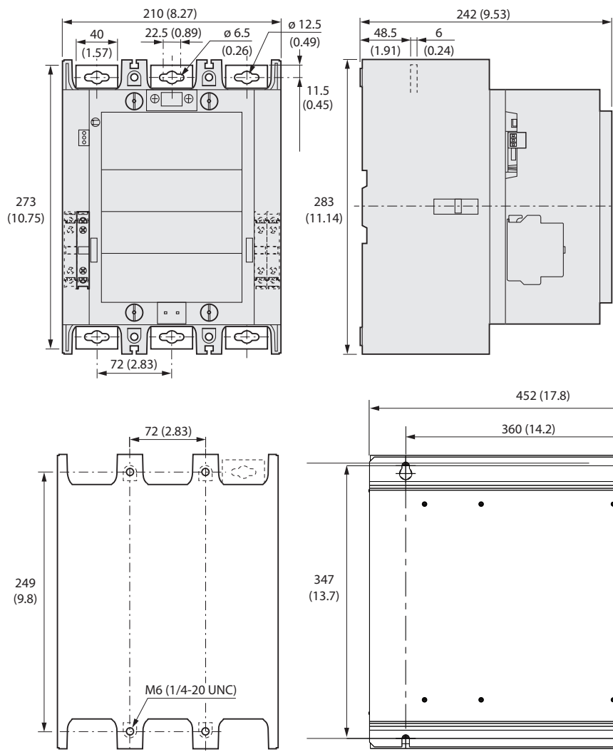
Figure 90 - 100-E1260 Contactors with PLC Input
