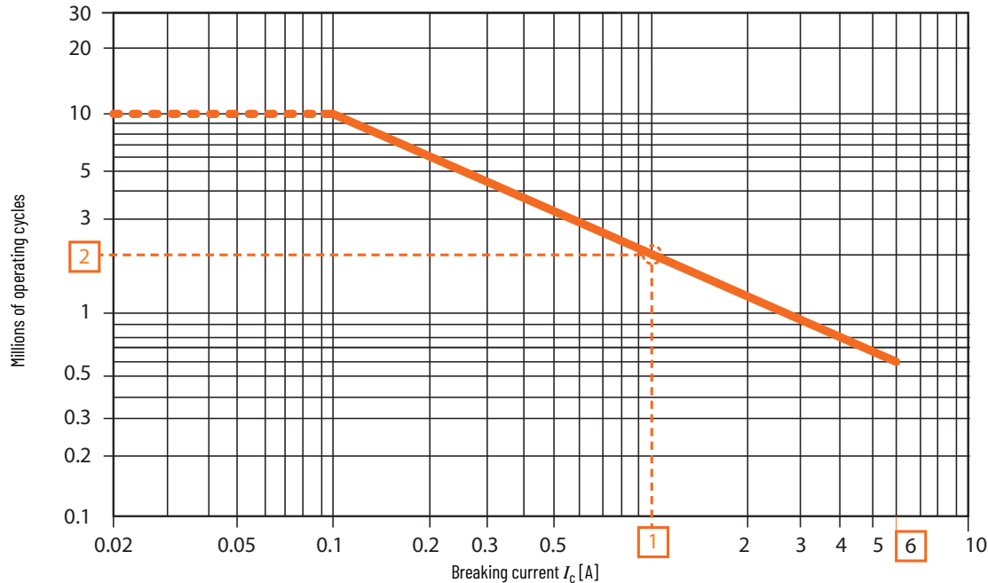
Figure 32 - Electrical durability for DC-13 utilization category - U_e \leq 250V
