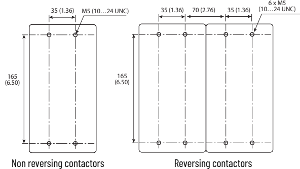
Figure 84 - 100-E265...100-E370 Contactors
