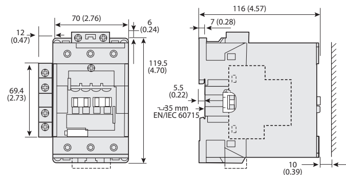
Figure 68 - 100-E80...100-E96 3-Pole Contactors with Side-mounted Auxiliary Contact
