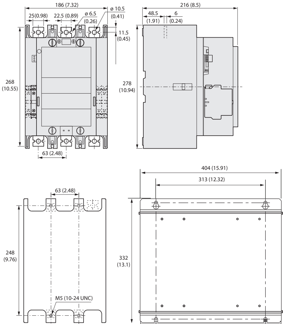
Figure 88 - 100-E400, 100-E460 Contactors with PLC Input
