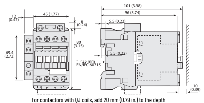
Figure 50 - 100-E26...100-E38 4-Pole Contactors with Standard Coils and Side-mounted Auxiliary Contact
