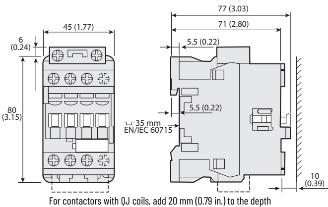
Figure 36 - 100-E09...100-E16 Contactors with Low-consumption Coils
