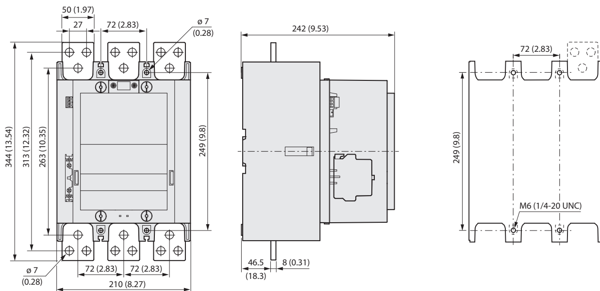
Figure 90 - 100-E1260 Contactors with PLC Input
