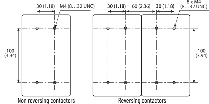
Figure 80 - 100-E190, 100-E205 Contactors
