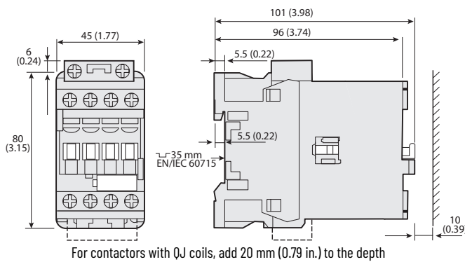
Figure 47 - 100-E26...100-E38 3-Pole Contactors with Standard Coils and Front-mounted Auxiliary Contact
