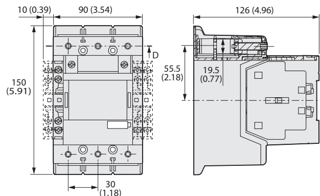
Figure 79 - Drilling Template for 116...146 A 3-Pole Contactors
