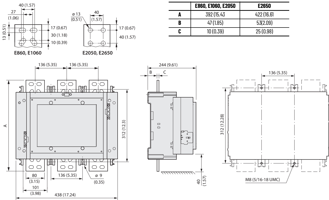
Figure 91 - 100-E860, 100-E1060, 100-E2050, 100-E2650 Contactors with PLC Input
