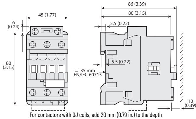
Figure 46 - 100-E26...100-E38 4-Pole Contactors with Low-consumption Coils
