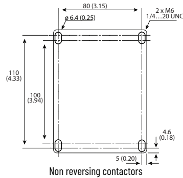
Figure 74 - Drilling Template for 80 A 4-Pole Contactors
