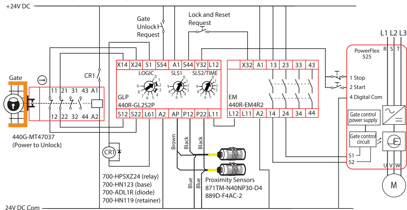
Figure 38 - Guard Locking Interlock with High Current Solenoid
