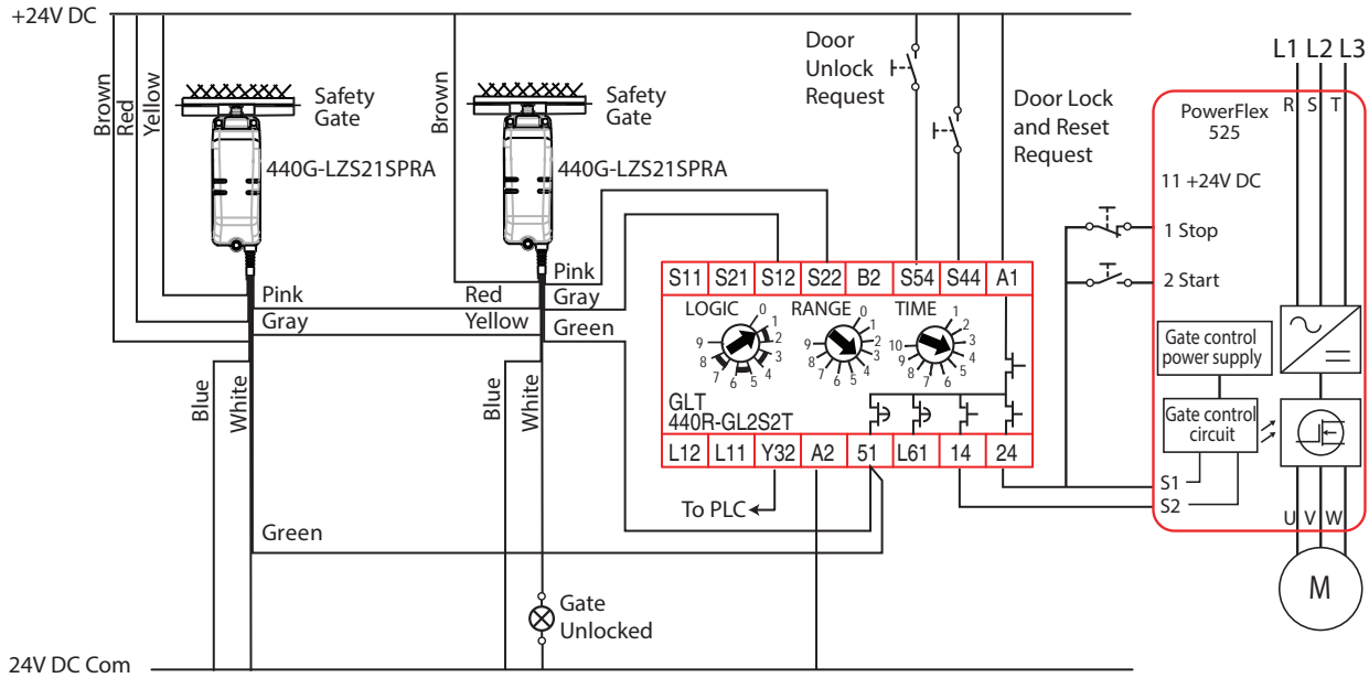
Figure 47 - Guard Locking with Time Delay
