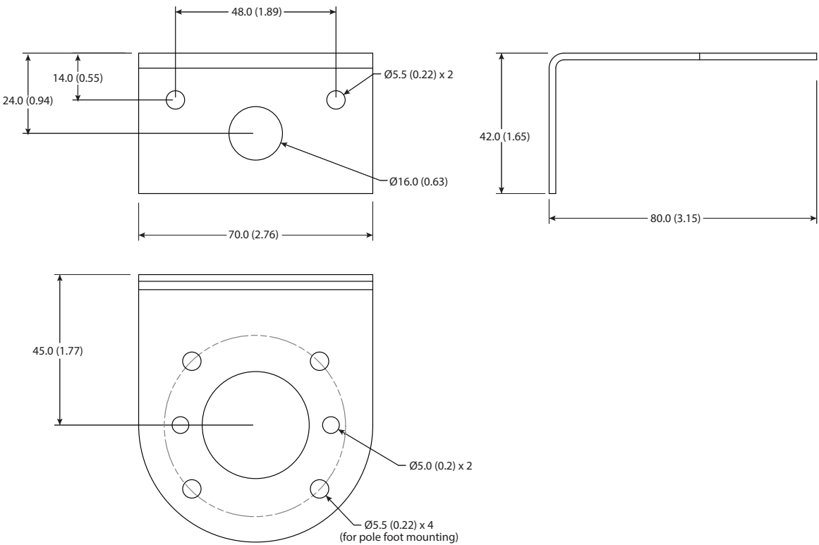
Catalog Number 855T-AVM Vertical Mount Bracket
