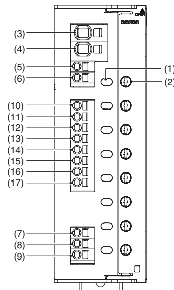
8-branch output type S8V-CP0824
